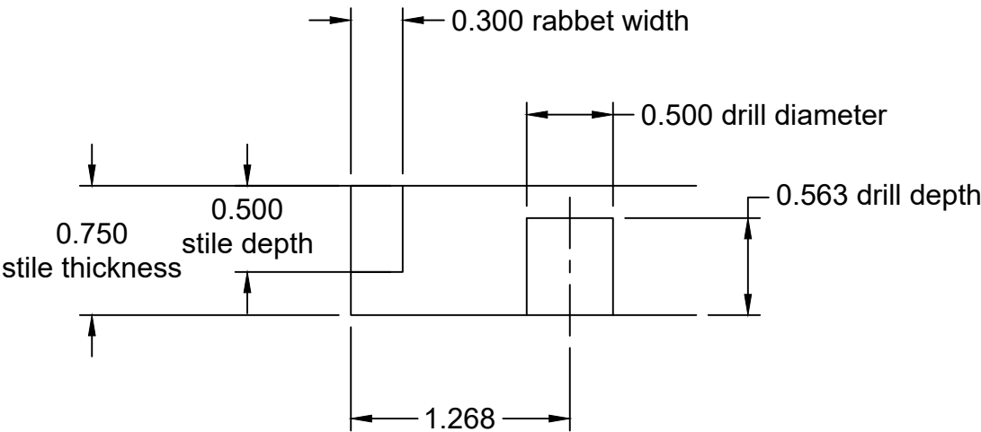
TYPICAL DETAIL
